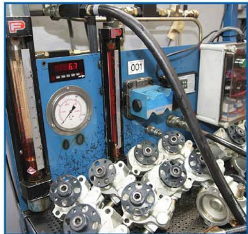
Remanufactured Power Steering Pumps Testing Station
