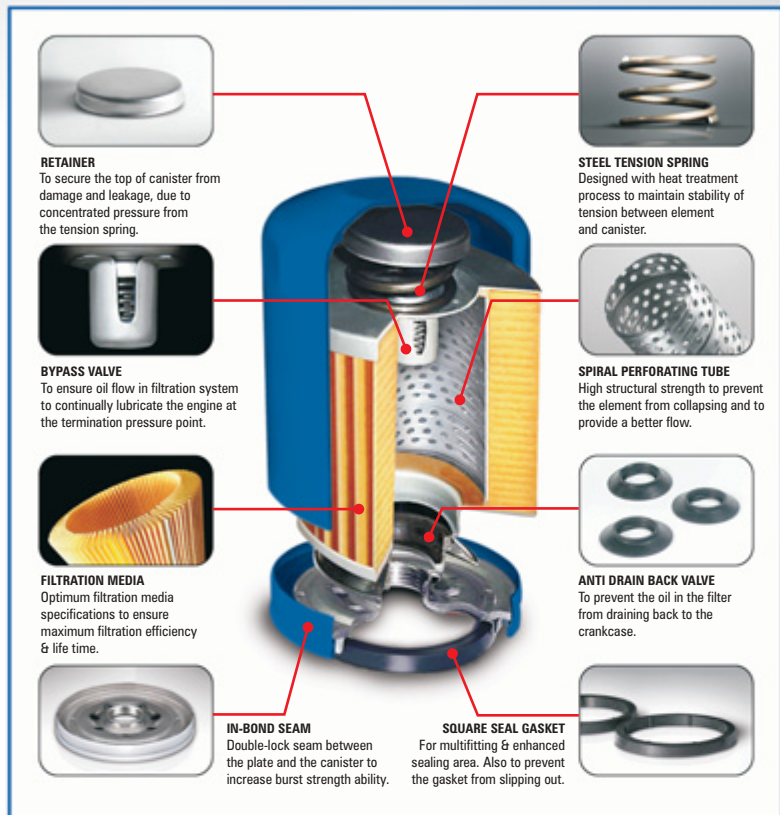
Cut Away of an ACDelco Oil Filter.
