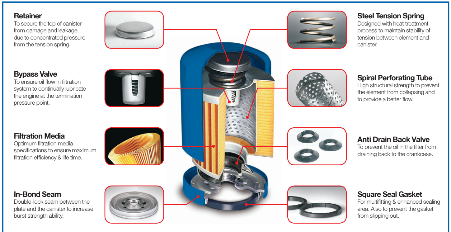
Cut Away of an ACDelco Oil Filter.
